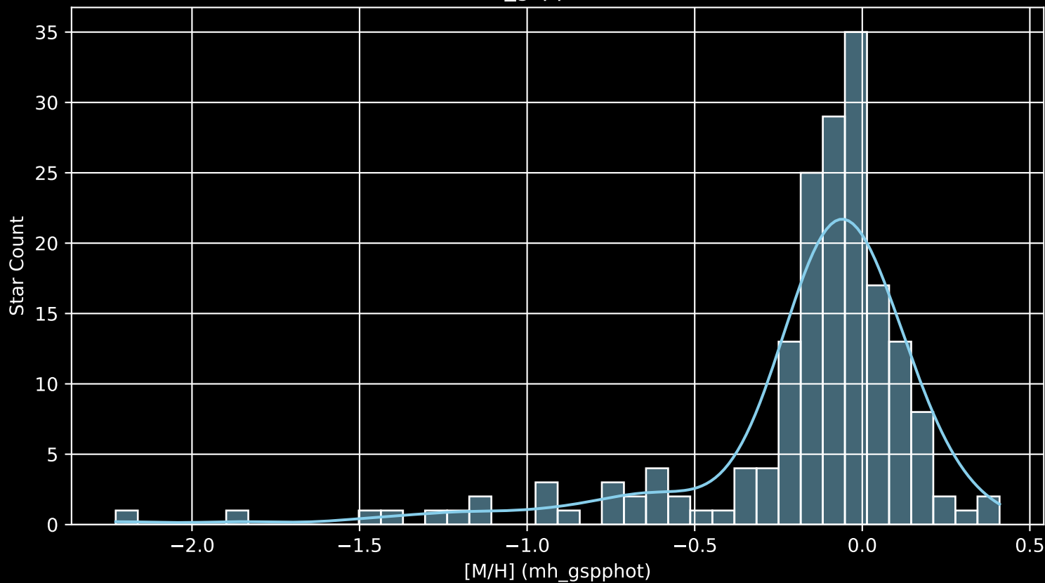
APOGEE DR17 Field: [143+04 [M/H] (mh_gspphot) (n= 178)
