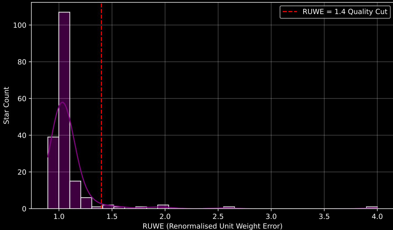
GAPOGEE DR17 Field [143+04] RUWE Distribution (n= 176)
