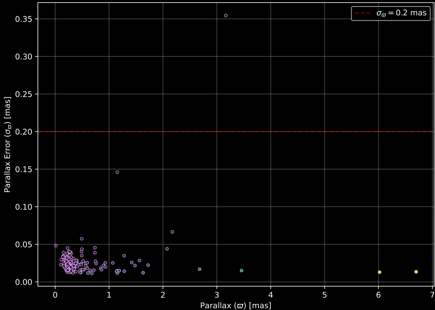
APOGEE DR17 Field: [143+04] Parallax Quality (n= 178)
