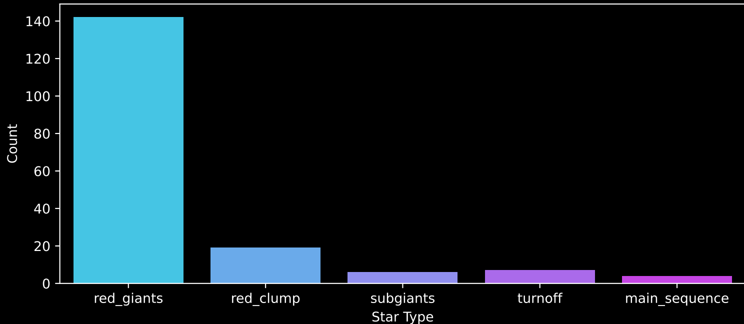
APOGEE DR17 Field: [143+04] Count plot of Star Type
