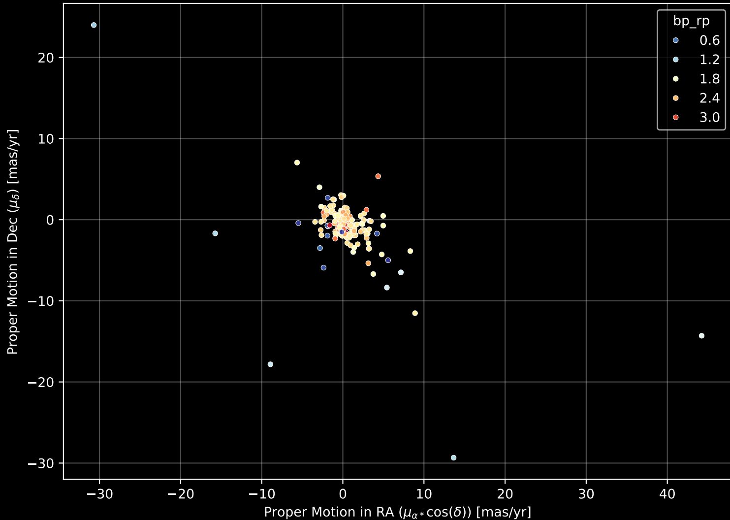
APOGEE DR17 Field: [143+04] Proper Motion Diagram (n= 178)
